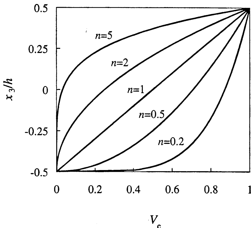
FIG. 1. Through-the-thickness distribution of the volume fraction of the ceramic phase in the functionally graded plate.
