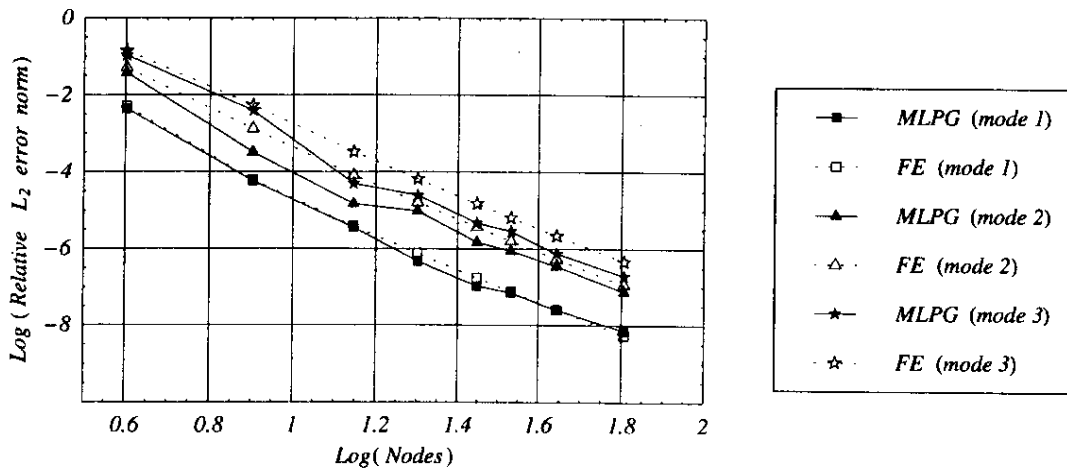
Figure 5 : Convergence rates of the three lowest modes in L_2 norm.
