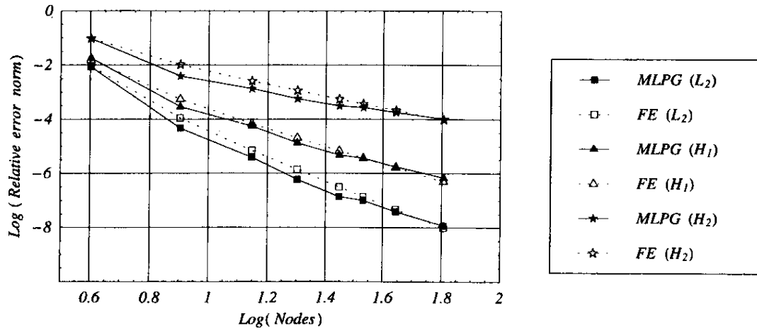
Figure 3 : For a uniformly loaded beam, convergence of the error norms with a decrease in the nodal spacing or an increase in the number of uniformly distributed nodes.
