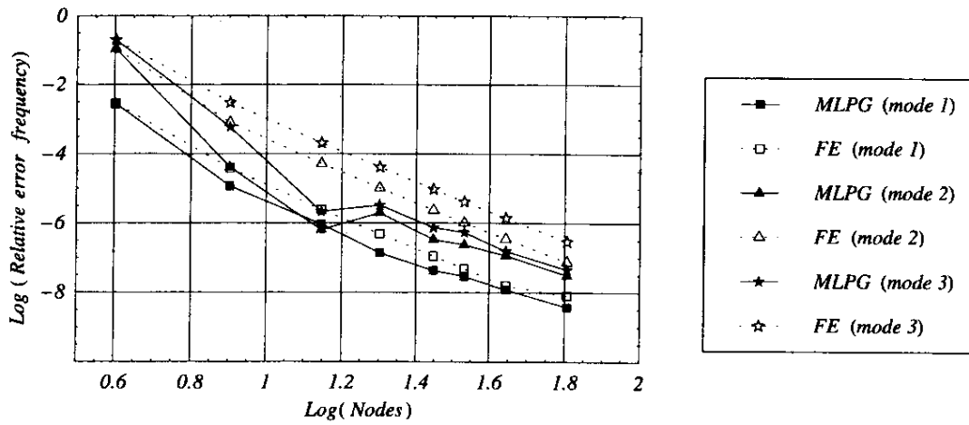
Figure 4 : Convergence rates of the first three natural frequencies.
