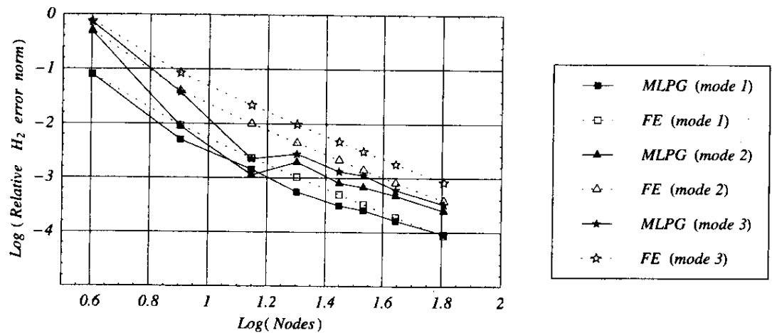
Figure 7 : Convergence rates of the three lowest modes in H_2 norm.
