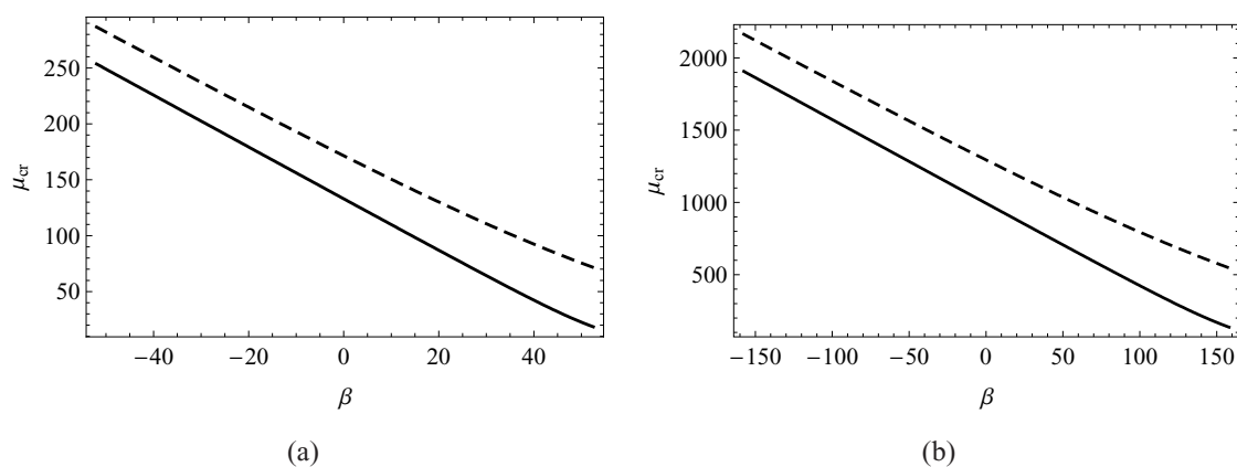
Figure 7. For \alpha = 1 (solid line) and \alpha = 4 (dashed line), variation with \beta of the critical van der Waals force parameter \mu_{\text{cr}} for (a) square plate and (b) rectangular plate with \varphi = 1/2 .
