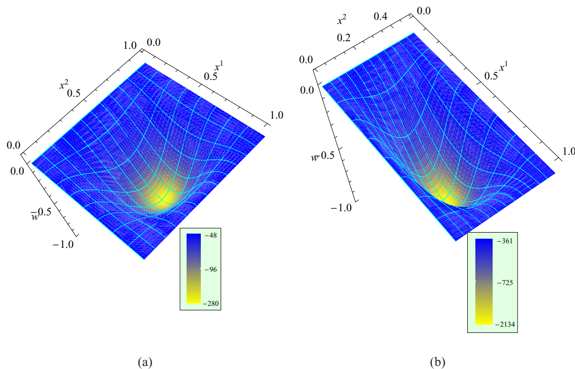
Figure 6. For \mu \simeq 0.3\mu_{\text{cr}} and \alpha = 4 , deformed shape of (a) the square plate with \lambda \simeq 200 and \|w\|_{\infty} \simeq 0.59 , and (b) rectangular plate with \varphi = 1/2 , \lambda \simeq 1500 and \|w\|_{\infty} \simeq 0.59 . Fringe plots of the van der Waals pressure are also displayed.
