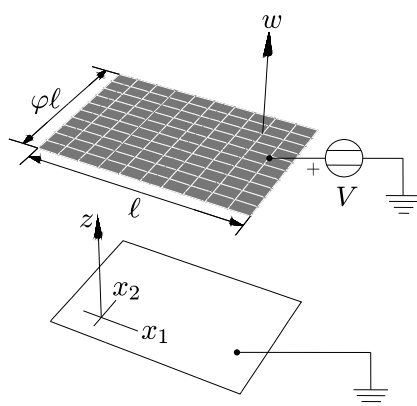
Figure 1. Sketch of an electrostatically actuated rectangular microplate.
